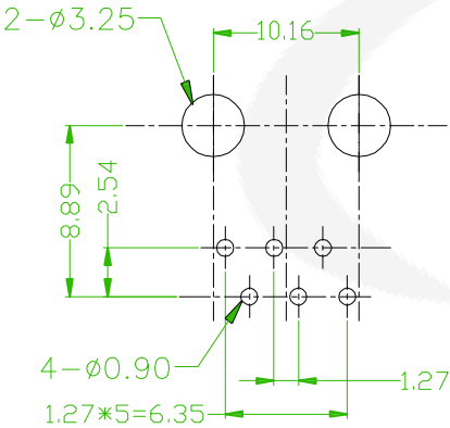
Recommended PCB Layout (PVB TOLERANCE±0.05)
