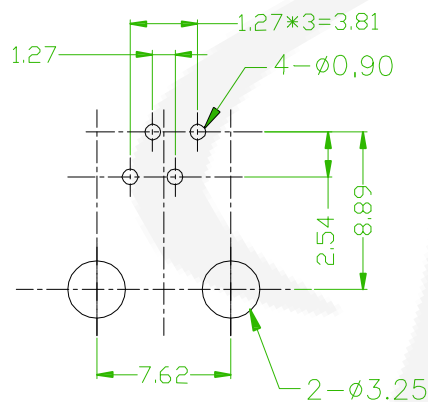
Recommended PCB Layout (PVB TOLERANCE±0.05)
