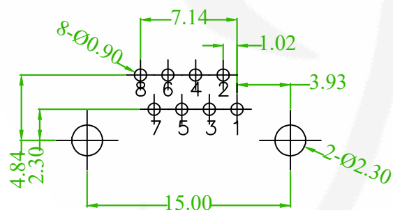
RECOMMENDED PCB LAYOUT (PCB TOLERANCE \pm 0.05 )
