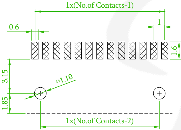
Recommended PCB Layout (PCB TOLERANCE ±0.1)
