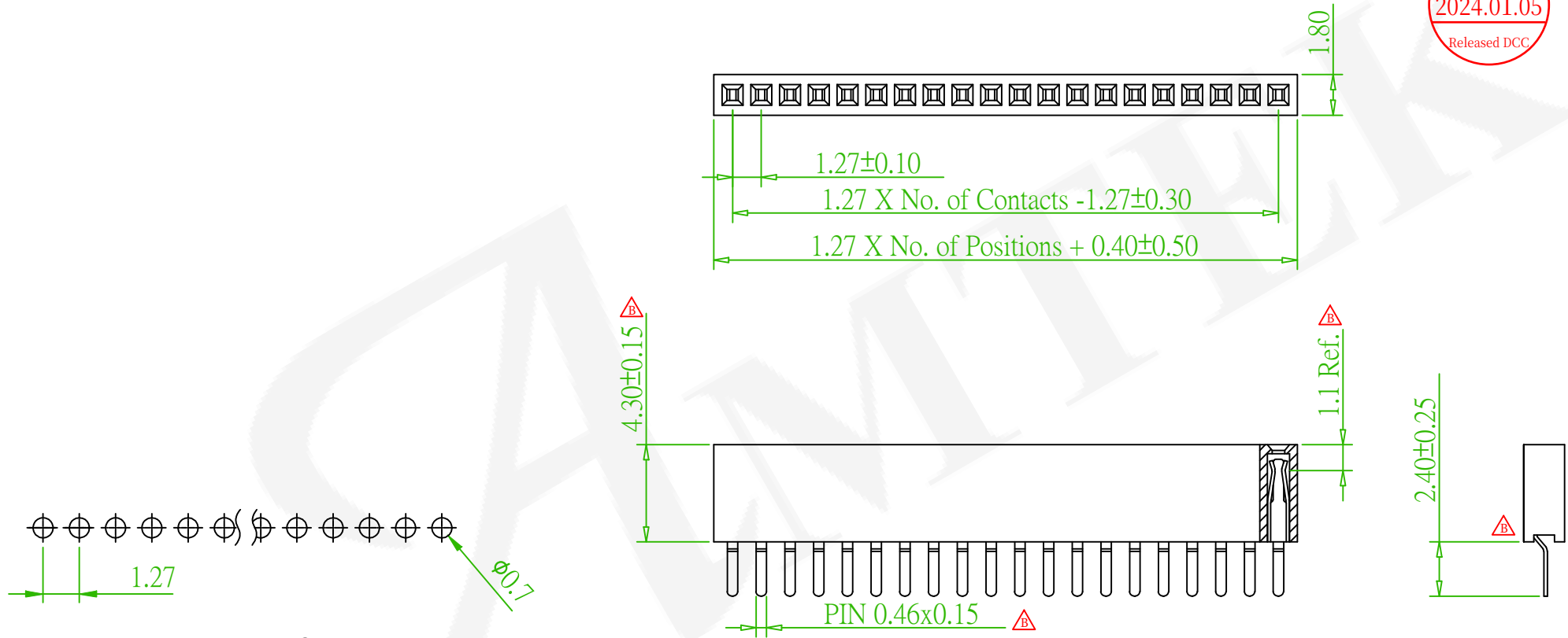
Recommended PCB Layout (PCB TOLERANCE ±0.05)
