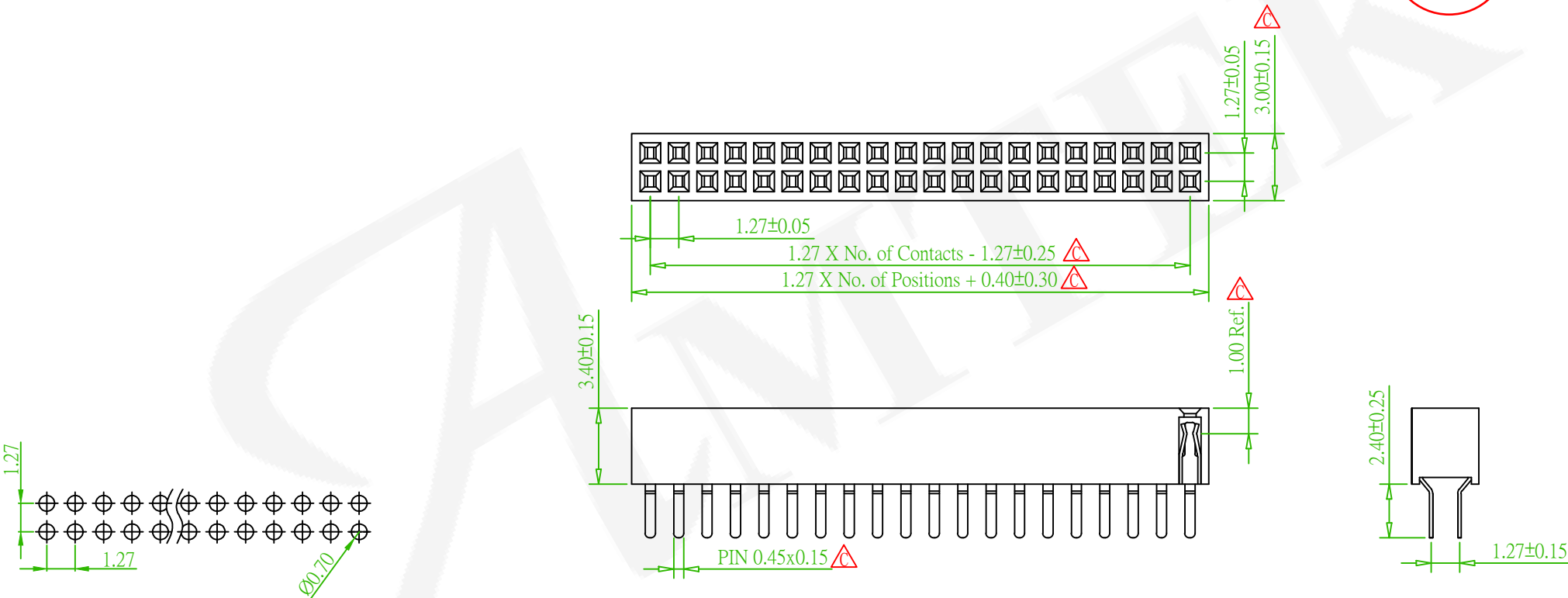
Recommended PCB Layout (PCB TOLERANCE ±0.05) ⚠
