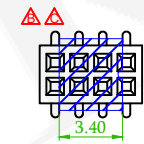
Special CAP for 2*2P 2*3P 2*4P W/O Bump
