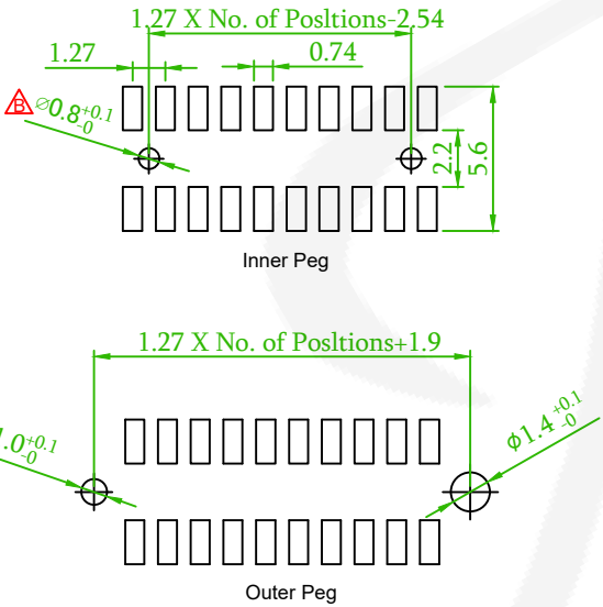
Recommended PCB Layout (PCB TOLERANCE ±0.05)
