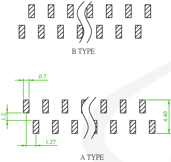
Recommended PCB Layout (PCB TOLERANCE \pm 0.05 )
