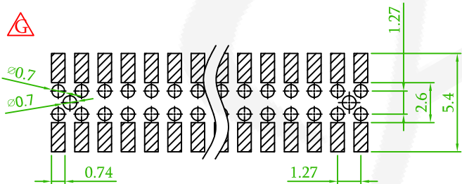
Recommended PCB Layout (PCB TOLERANCE ±0.05)
