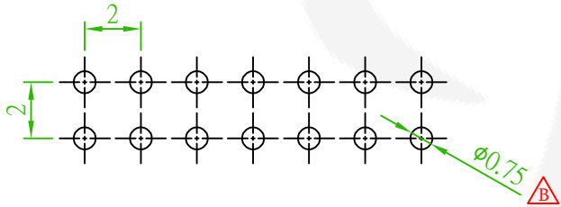
Recommended PCB Layout (PCB TOLERANCE ±0.05) △B
