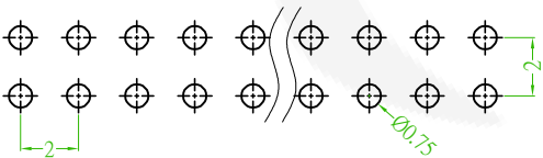
Recommended PCB Layout (PCB TOLERANCE ±0.05)
