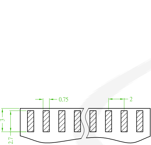
Recommended PCB Layout (PCB TOLERANCE ±0.05)
