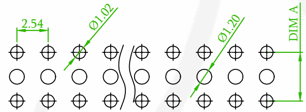
RECOMMENDED PCB LAYOUT (PCB TOLERANCE ±0.05)
