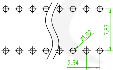
Recommended PCB Layout (PCB TOLERANCE ±0.1)
