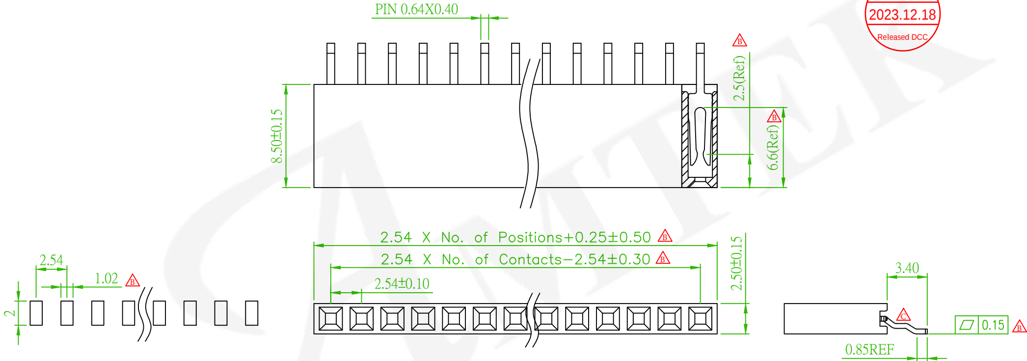
Recommended PCB Layout (PCB TOLERANCE ±0.05)
