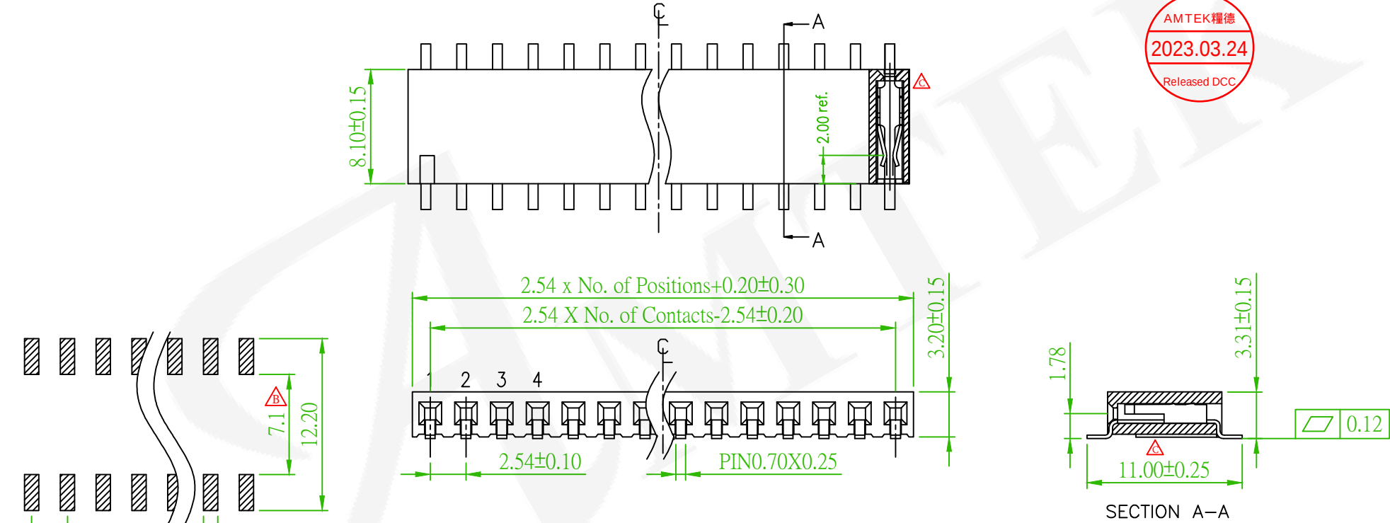
Recommended PCB Layout (PCB TOLERANCE \pm 0.1 )
