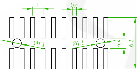
RECOMMENDED PCB LAYOUT (PCB TOLERANCE \pm 0.05 )
