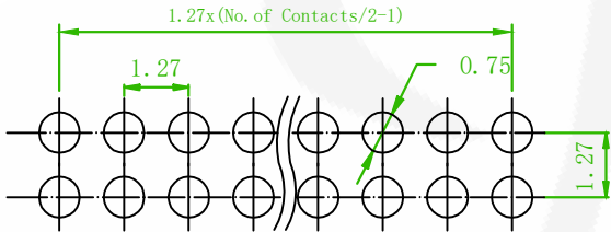
Recommended PCB Layout (PCB TOLERANCE ±0.05)
