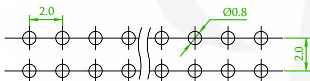
RECOMMENDED PCB LAYOUT (PCB TOLERANCE ±0.05)
