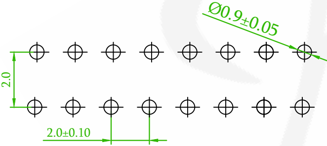
RECOMMENDED PCB LAYOUT (PCB TOLERANCE ±0.05)
