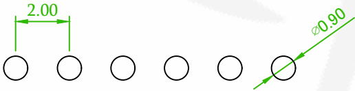
RECOMMENDED PCB LAYOUT (PCB TOLERANCE ±0.05)
