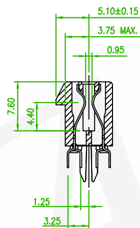
SECTION F-F
