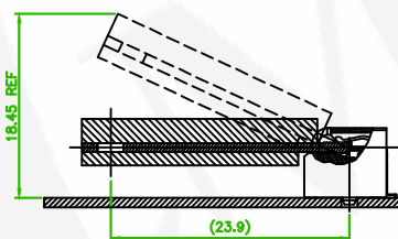
EJECT HEIGHT FOR HALF CARD
