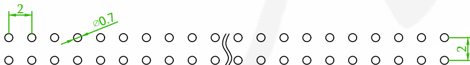
RECOMMENDED PCB LAYOUT (PCB TOLERANCE \pm 0.05 )
