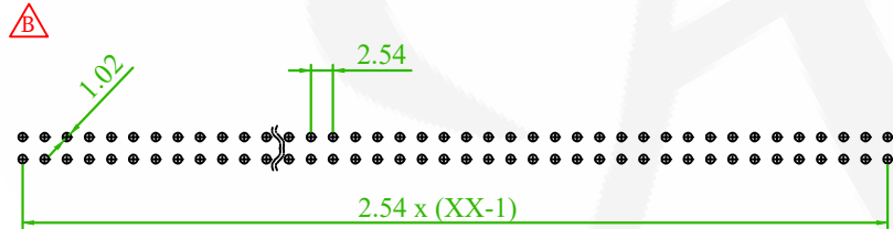
RECOMMENDED PCB LAYOUT (PCB TOLERANCE ±0.05)
