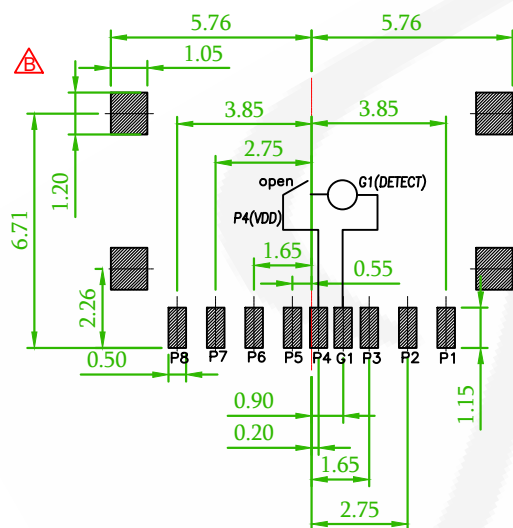
RECOMMENDED PCB LAYOUT (PCB TOLERANCE ±0.05)
