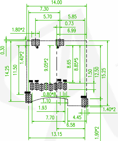
RECOMMENDED PCB LAYOUT (TOLERANCE ±0.05)
