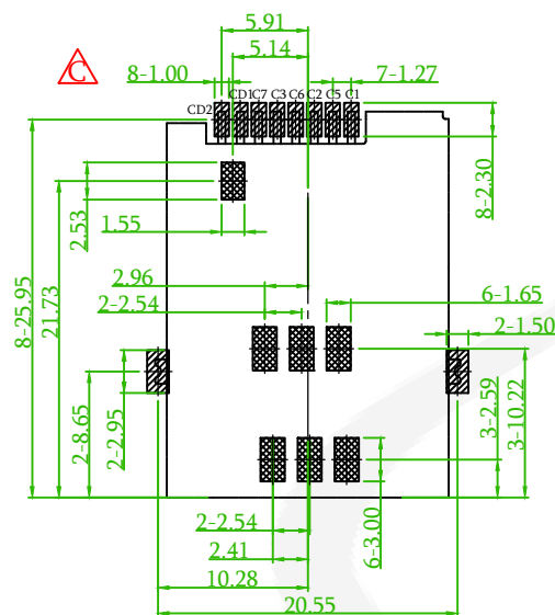
RECOMMENDED PCB LAYOUT (PCB TOLERANCE \pm 0.05 )
