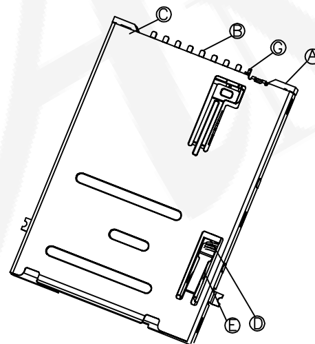
SIM CARD DIMENSION
