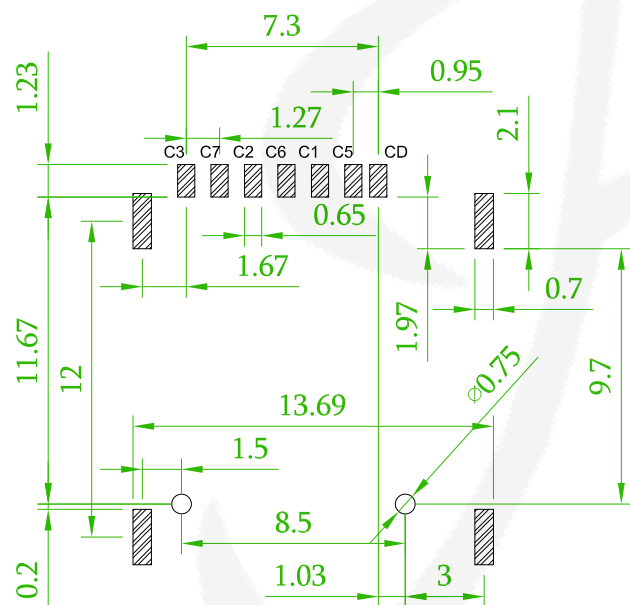
Recommended PCB Layout (PCB TOLERANCE ±0.05)
