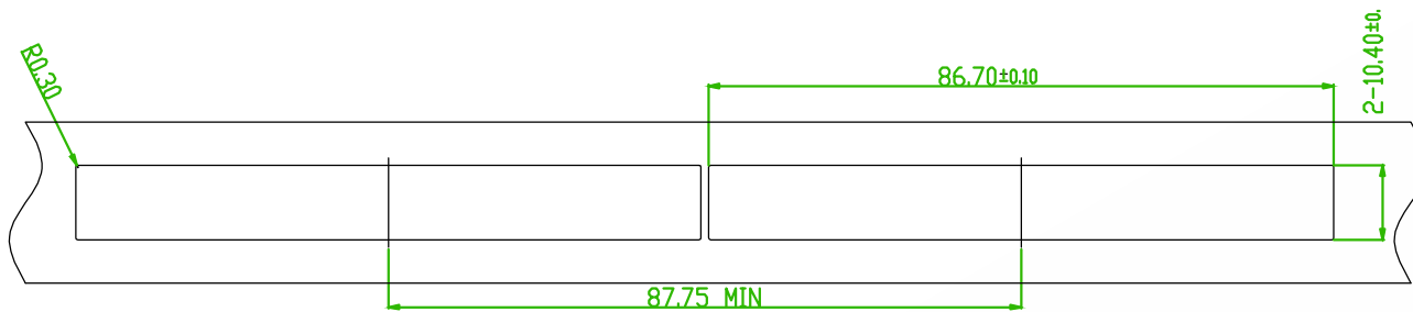
RECOMMENDED BEZEL CUT-OUT SINGLE SIDED APPLICATIONS
