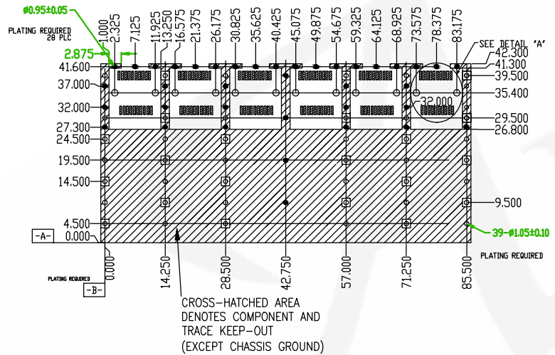
RECOMMENDED PCB CONFIGURATION WITH KEEP-OUT AREAS PFLY TO PFLY APPLICATIONS
