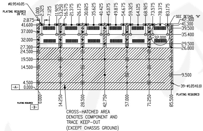
RECOMMENDED PCB CONFIGURATION WITH KEEP-OUT AREAS BFLY TO BFLY APPLICATIONS
