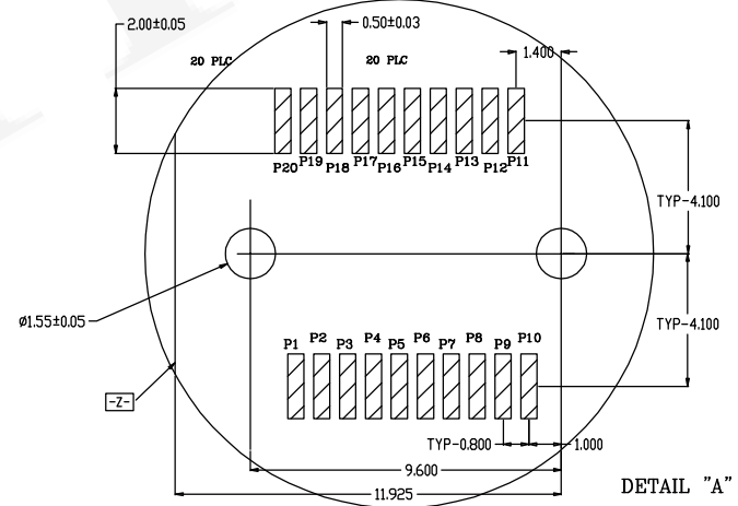
RECOMMENDED PCB CONFIGURATION WITH KEEP-OUT AREAS SINGLE SIDED APPLICATIONS
