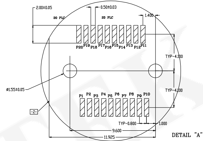
RECOMMENDED PCB CONFIGURATION WITH KEEP-OUT AREAS SINGLE SIDED APPLICATIONS
