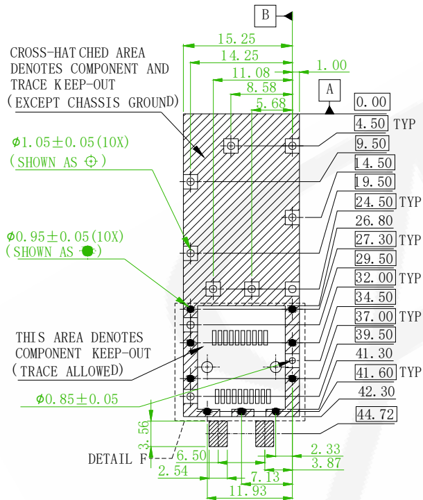
PCB LAYOUT (TOP VIEW) PCB TOLERANCES: +/-0.05
