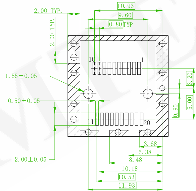
DETAIL F
