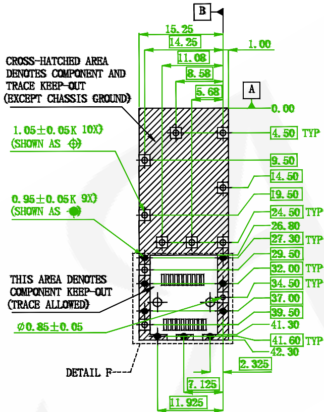
PCB LAYOUT (TOP VIEW) PCB TOLERANCES: +/- 0.05
