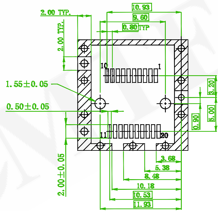
DETAIL F
