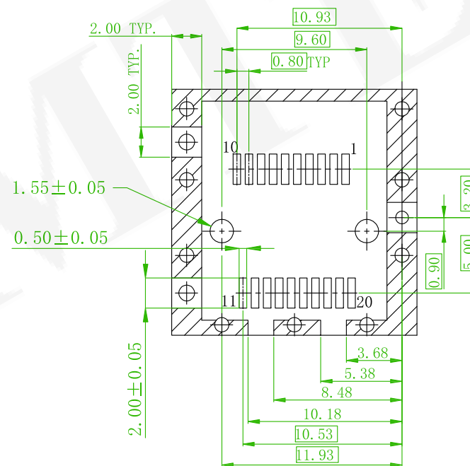
DETAIL F
