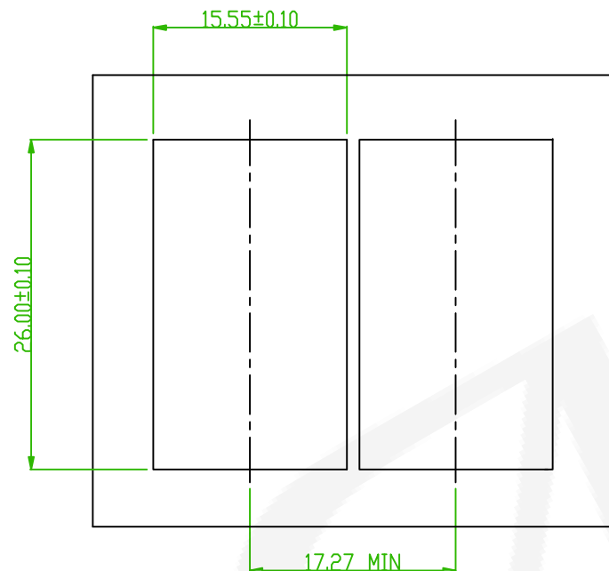
BEZEL CUT-OUT CENTER SPACING DETAIL BEZEL THICKNESS:0.8-2.6
