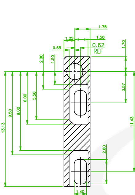
KEEP-OUT ZONE DETAIL
