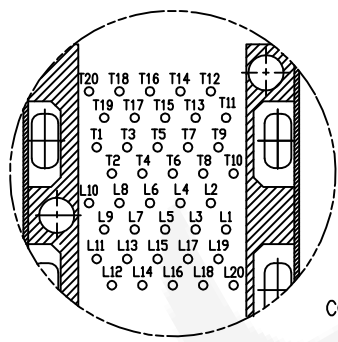
KEEP-OUT ZONE DETAIL
