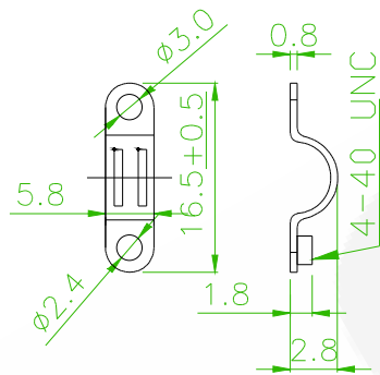
(B) RETAINER
