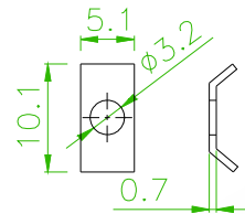
(E) WASHER
