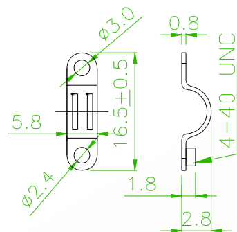
(B)RETAINER
