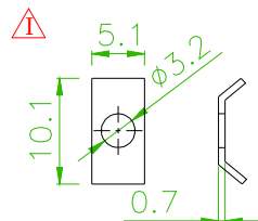
(E)WASHER
