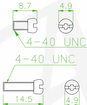
(C)SCREW
