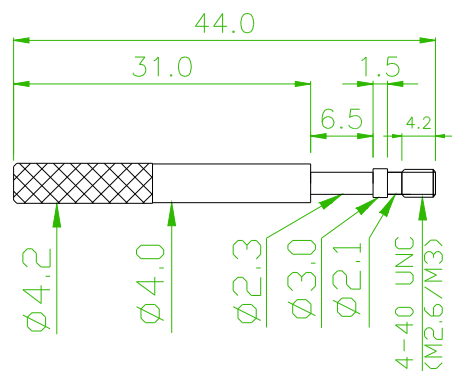
(A)THUMBSCREWS
