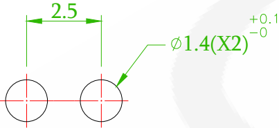
MOUNTING HOLE
