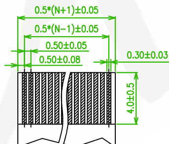
FPC/FFC T=0.30±0.03mm
