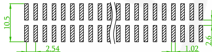
RECOMMENDED PCB LAYOUT (PCB TOLERANCE \pm 0.05 )
