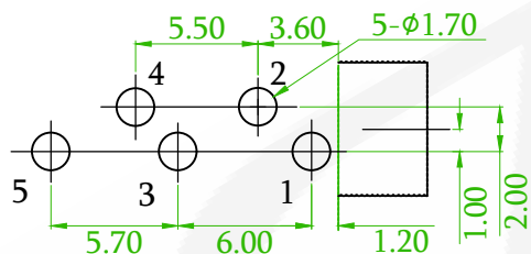
RECOMMENDED PCB LAYOUT (PCB TOLERANCE \pm 0.05 ) (BOTTOM VIEW)
