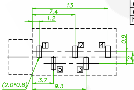
RECOMMENDED PCB LAYOUT (PCB TOLERANCE ±0.05)COPPER-SIDE VIEW
