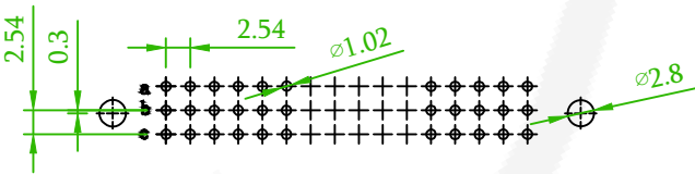
RECOMMENDED PCB LAYOUT (PCB TOLERANCE ±0.05)
