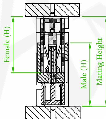
Mated Drawing (REF.)
