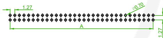
RECOMMENDED PCB LAYOUT (PCB TOLERANCE ±0.05)
