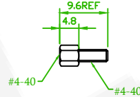
57WHSSXM-XXXBXXA-02 Thread Insert #4-40 + Jack Screw #4-40 Attached
