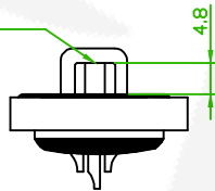
57WHSSXM-XXXCXXA-02 Thread Insert #4-40 UNC +Jack Screw #4-40 UNC Removable
