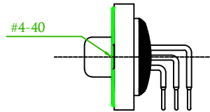
57WHDRXM-XXXAXXA-02 Thread Insert #4-40
