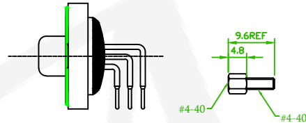
57WHDRXM-XXXBXXXA-02 Thread Insert #4-40 + Jack Screw #4-40 Attached
