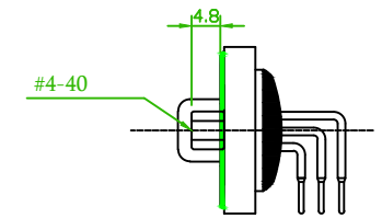
57WHDRXM-XXXCXXXA-02 Thread Insert #4-40 UNC + Jack Screw #4-40 UNC Removable
