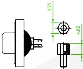
57WDDSXM-XXBBXXBA-01 THREAD INSERT #4-40 + JACK SCREW #4-40 ATTACHED
