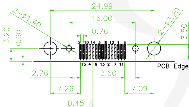
Recommended PCB Layout (PCB TOLERANCE \pm 0.05 )
